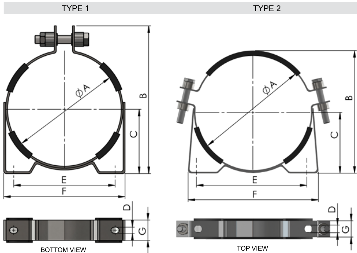
MOUNTING COLLARS FOR BLADDER ACCUMULATORS*
